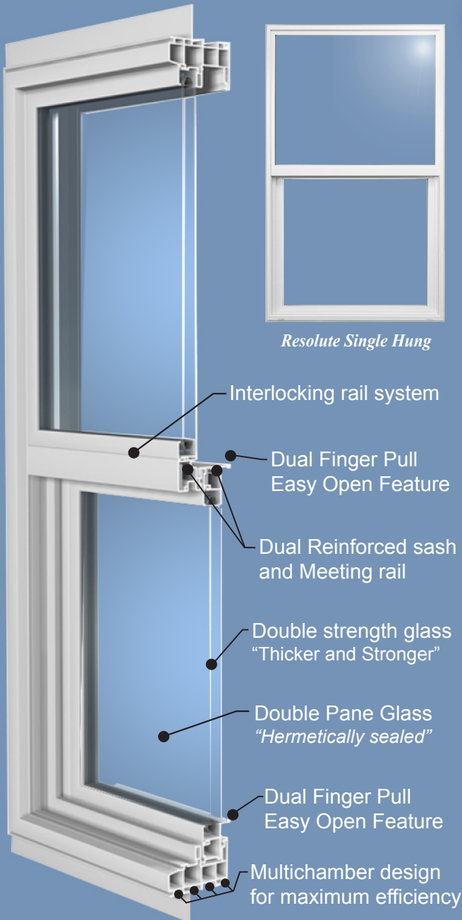
Single Hung Resolute Window Cross-section
