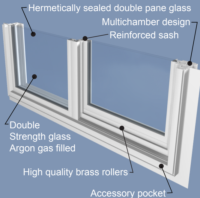
Three Lite Horizontal Slider
