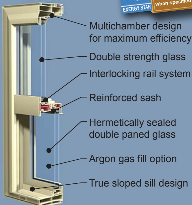
Single Hung Window Cross-section in Almond
