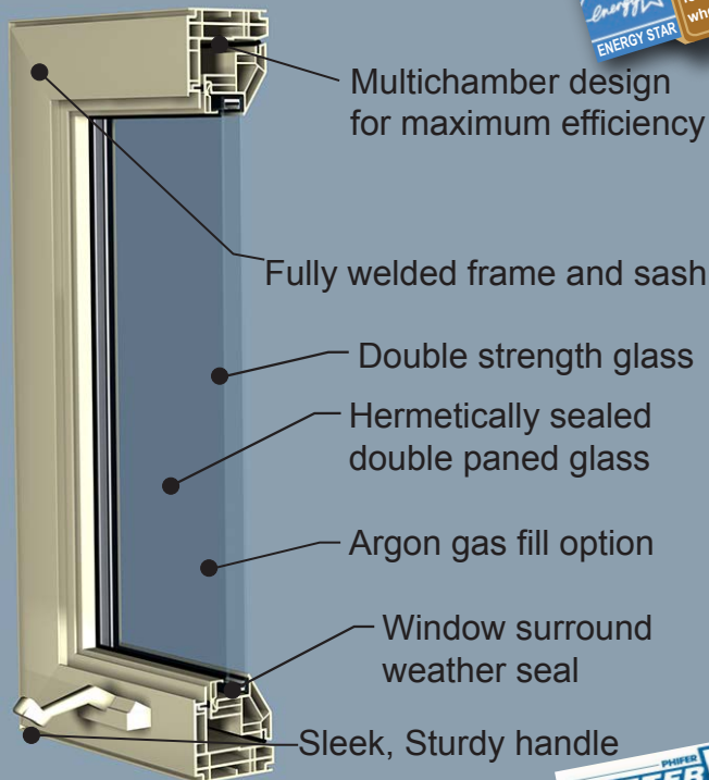
Casement Window Cross-section in Almond
